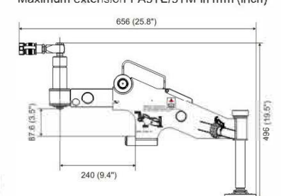
Maximum extension FA9TE/9TM in mm (inch)
