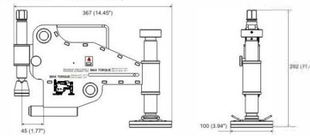
Minimum extension FA4TM in mm (inch)
