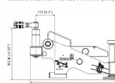
Minimum extension FA9TE/9TM in mm (inch)
