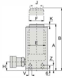
Optional Bolt-on Tilt Saddle Dimensions (mm)
