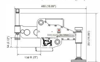
Maximum extension FA4TM in mm (inch)
