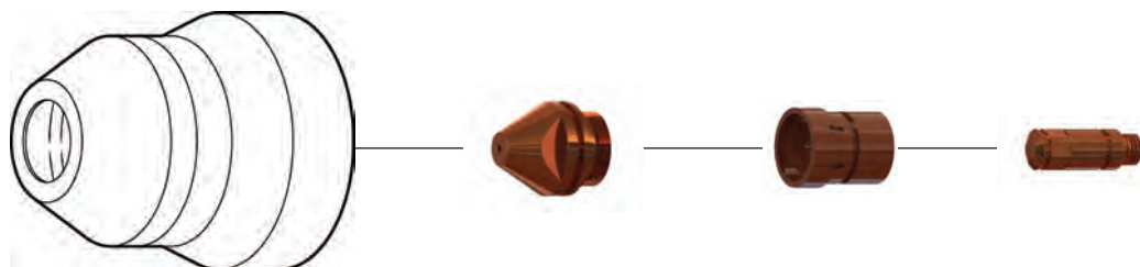
Shield Cup *9-6075
